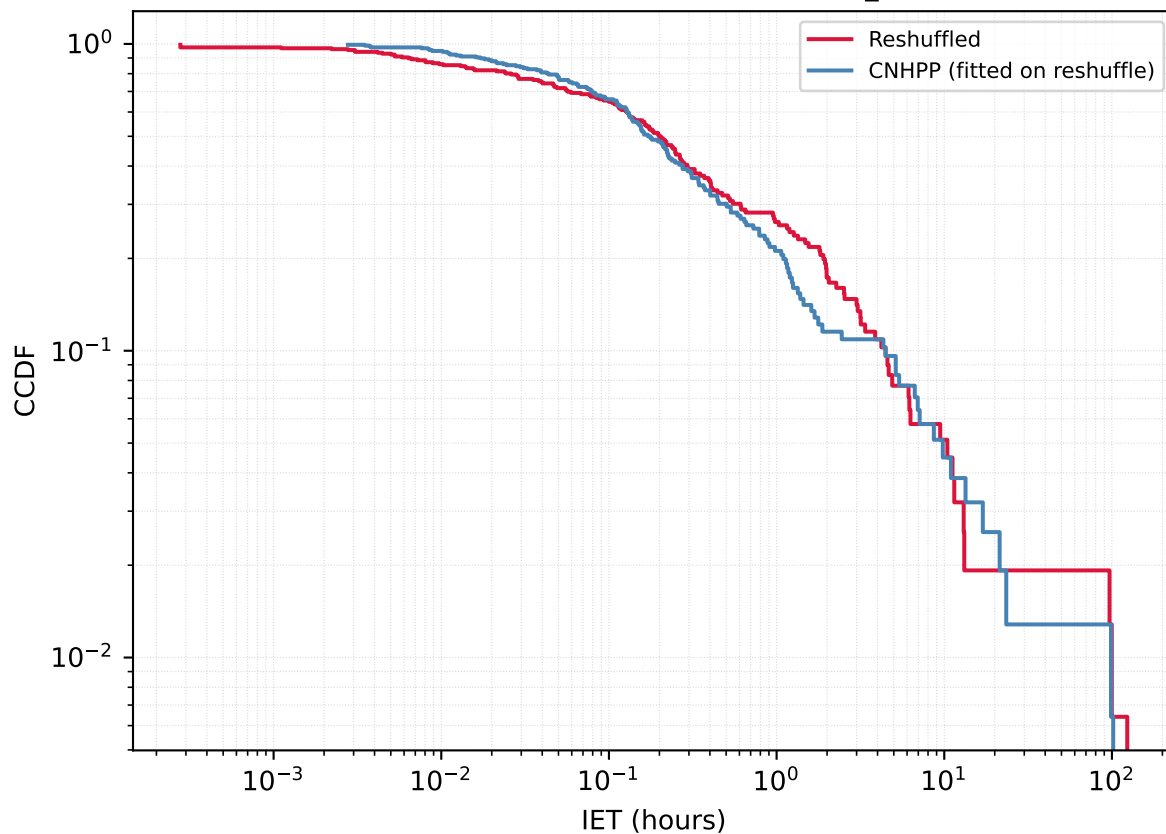
User 1354320169 - Reshuffled vs CNHPP A_{\text{fit}}=0.4376
